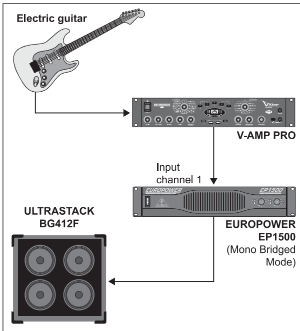
Fig. 3.5: Mono-bridged mode
